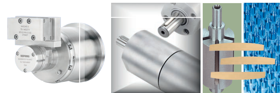
Air motor-gear-valve, a system for the paper industry made of stainless steel; sealed stainless steel motors and high performance vanes
