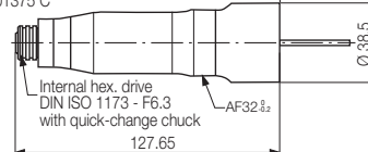
Shut-off clutch cpl. 401375 C
