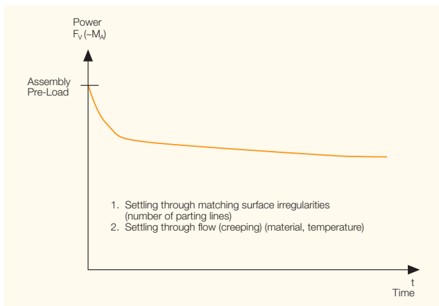
Seating processes
