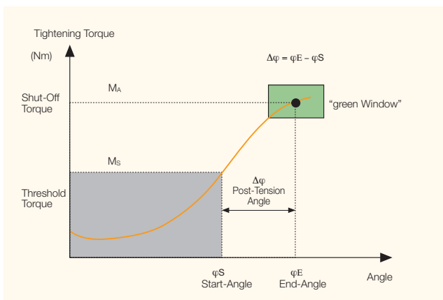
Angle-controlled tightening
