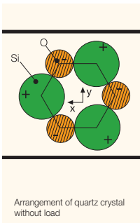
Function principle of the piezoelectric transducers
