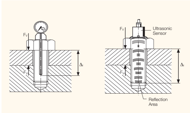
Length measurement
