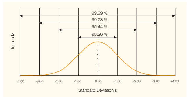
Gaussian standard distribution
