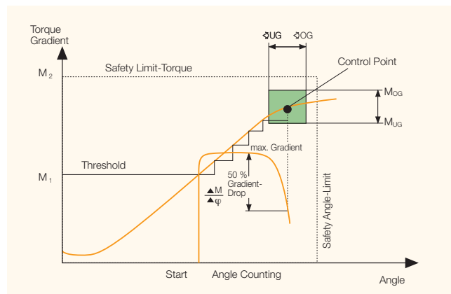
Limit-value controlled tightening
