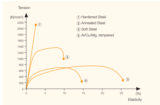
Hooke's Tension-/Elasticity-Diagram
